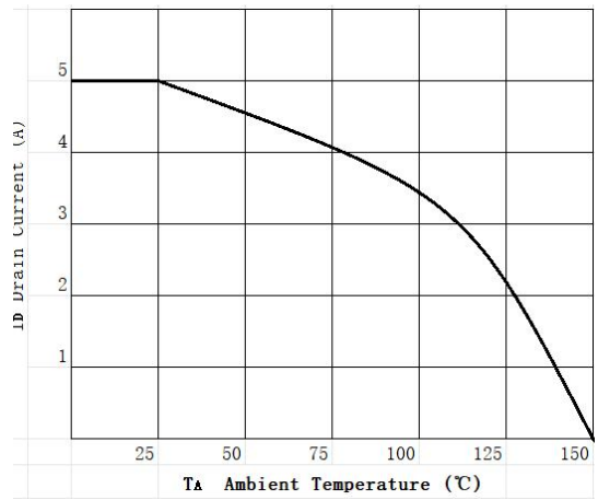
Figure 4: Drain Current vs. Temperature
