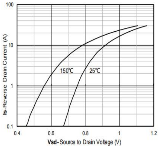
Figure 9: Diode Characteristics
