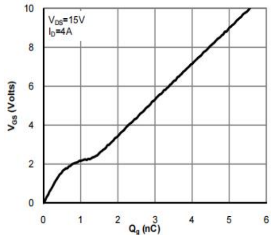
Figure 6: Gate-Charge Characteristics
