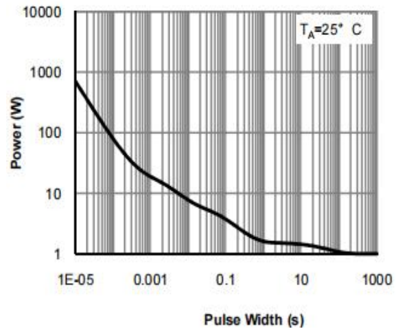
Figure 8: Power Rating
