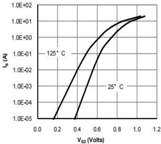
Figure 9: Diode Characteristics
