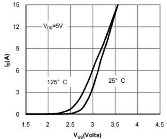
Figure 4: Transfer Characteristics
