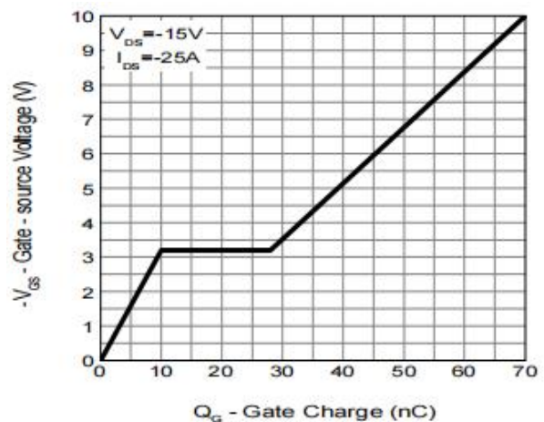
Figure 6: Gate-Charge Characteristics
