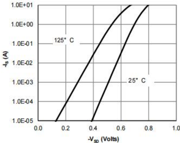
Figure 3: Diode Characteristics
