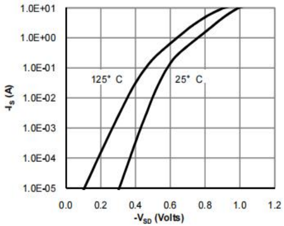
Figure 7: Diode Characteristics
