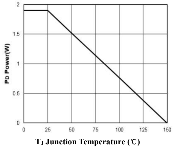
Figure 8: Power Dissipation
